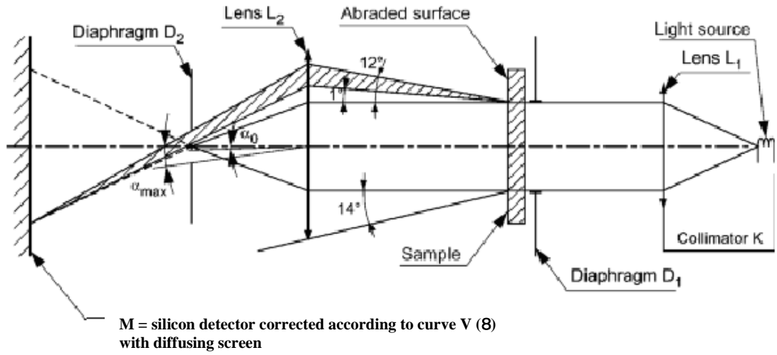
Figure 1: Test equipment
